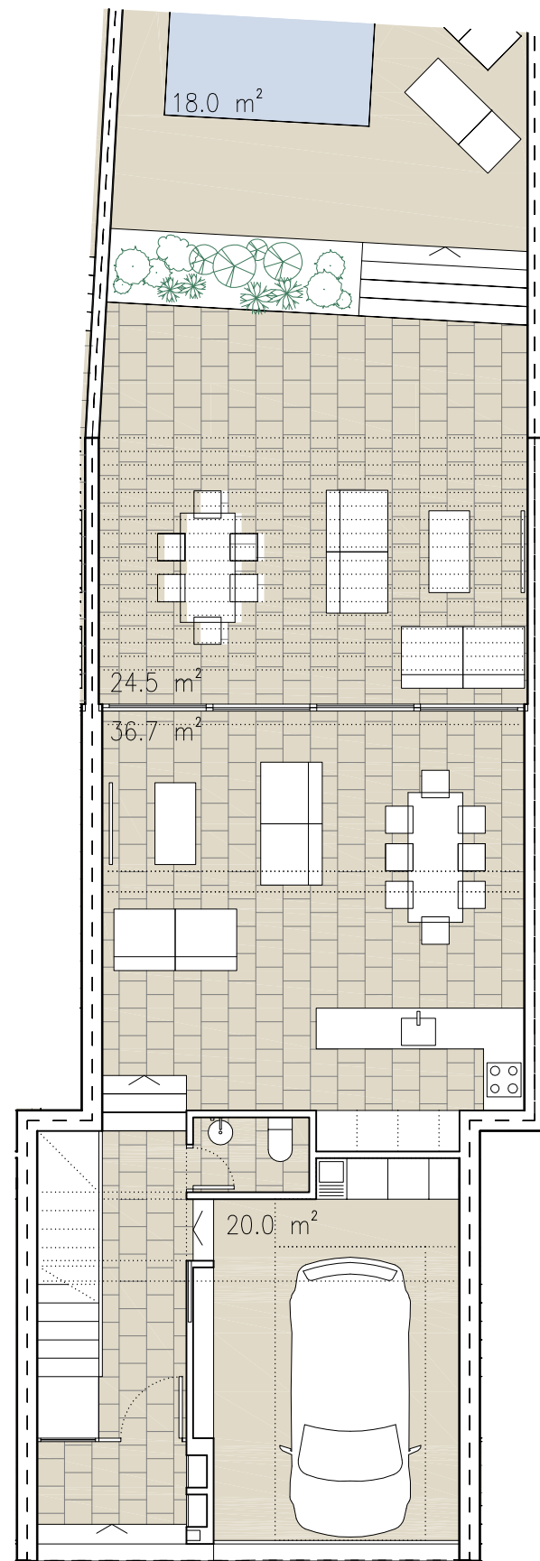
PLANTA BAJA / GROUND FLOOR 1/100
